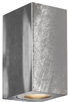
Canto Maxi Kubi 2 49731031 Galvanized | Galvanized steel Excl. GU10 | Max. 2x28W H: 16 cm | W: 8,7 cm
