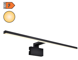
Marlee 80 2510351003 Black | Aluminium LED Module 11,5W | 1000lm | 3000K H: 9,6 cm | W: 80 cm | L: 80 cm
