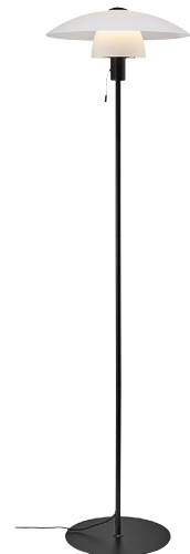
Verona 2010884001 Black | Glass Excl. E27 | Max. 25W H: 150 cm | Ø: 40 cm
