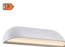
Front 26 84081001 White | Metal LED Module 9,8W | 650lm | 3000K H: 6,8 cm | W: 26 cm
