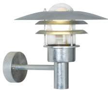
Lønstrup 32 71411031 Galvanized | Galvanized steel Excl. E27 | Max. 60W H: 28,5 cm | Ø: 32 cm
